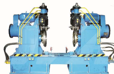
Seaming machine
