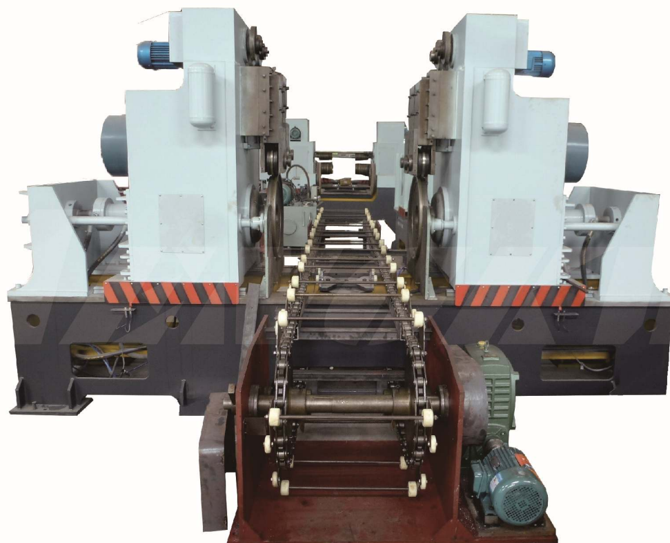
Flanging machine
